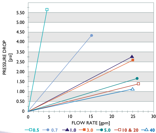
Flow Characteristics
